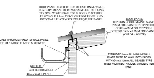
ROOF TO GUTTER DETAIL:
