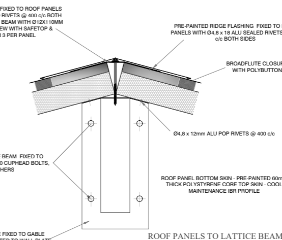
ROOF PANELS TO LATTICE BEAM DETAIL
