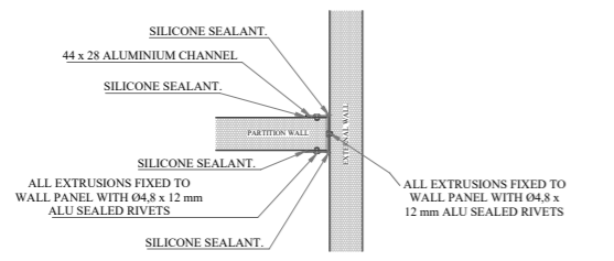
G. INTERNAL PARTITION WALL TO EXTERNAL WALL FIXING DETAIL
