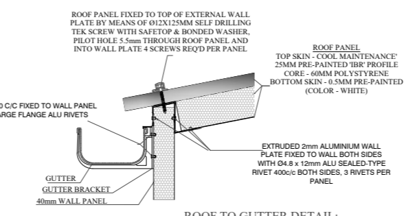
ROOF TO GUTTER DETAIL:
