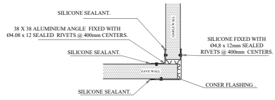
WALL TO WALL OUTSIDE CORNER FIXING DETAIL:
