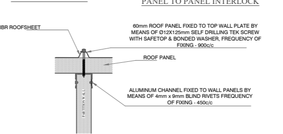
INTERNAL PARTITION WALL TO ROOF FIXING DETAIL
