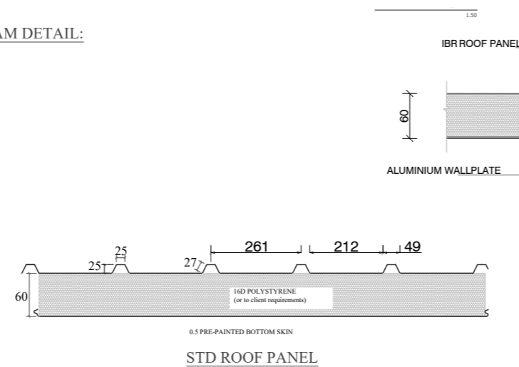
ROOF PANEL FIXED TO TOP OF EXTERNAL WALL PLATE BY MEANS OF Ø12X125MM SELF DRILLING TEK SCREW WITH SAFETOP & BONDED WASHER, PILOT HOLE 5.5mm THROUGH ROOF PANEL AND INTO WALL PLATE 4 SCREWS REQ'D PER PANEL
