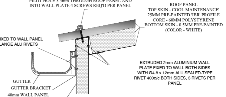
ROOF TO GUTTER DETAIL:
