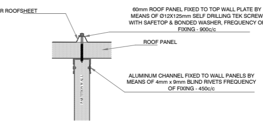
INTERNAL PARTITION WALL TO ROOF FIXING DETAIL
