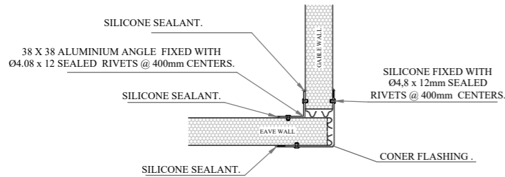
WALL TO WALL OUTSIDE CORNER FIXING DETAIL:
